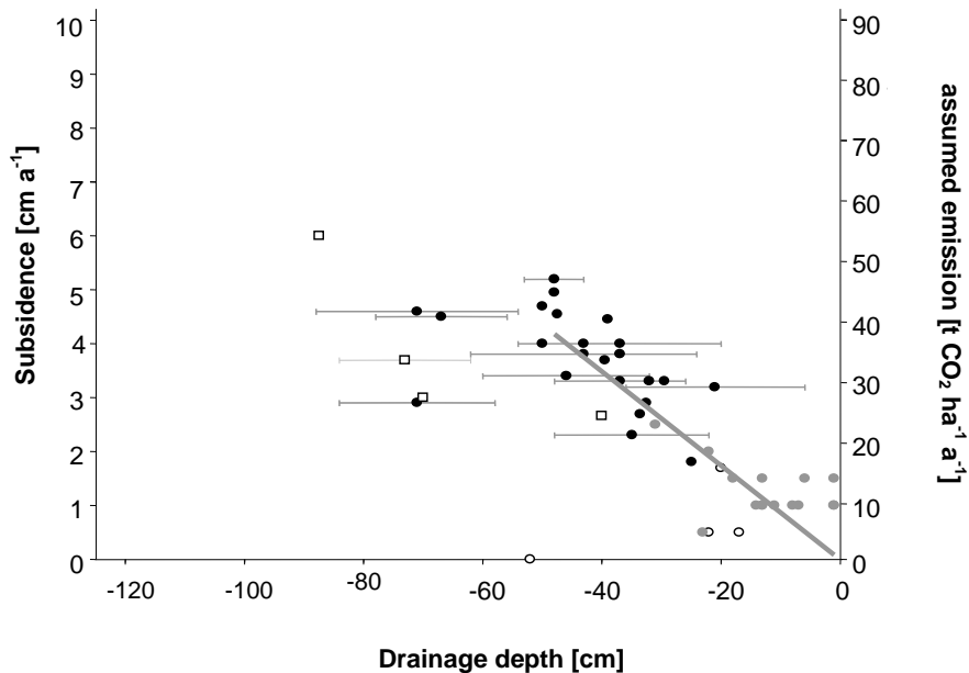
Figure 2.4.3. Relation between drainage depth and CO 2 emissions from peat decomposition in tropical peat swamps 48 . Rate of subsidence in relation to mean annual water level below surface. Horizontal bars indicate standard deviation in water table (where available). Open circles denote unused, drained forested sites. Land use: (□) agriculture, (●) oil palm (recorded 13 to 16 or 18 to 21 years after drainage), (●) degraded open land in the Ex Mega Rice Project area, recorded ~10 to ~12 years after drainage, (○) drained forested plots, recorded ~10 to 12 years after drainage. The slope of the line represents 0.9 t CO 2 /ha emitted per 1 cm drained.
